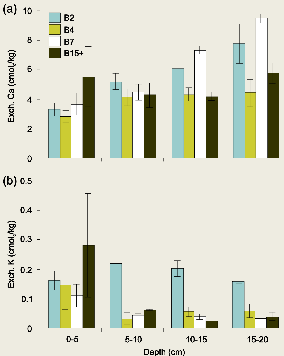
Figure 3.3. Mean ( \pm 1 St. Error) exchangeable (a) Ca and (b) K at four depths in peat burned <2 years (B2), 4 years (B4), 7 years (B7) and >15 years (B15+) prior to sampling.
