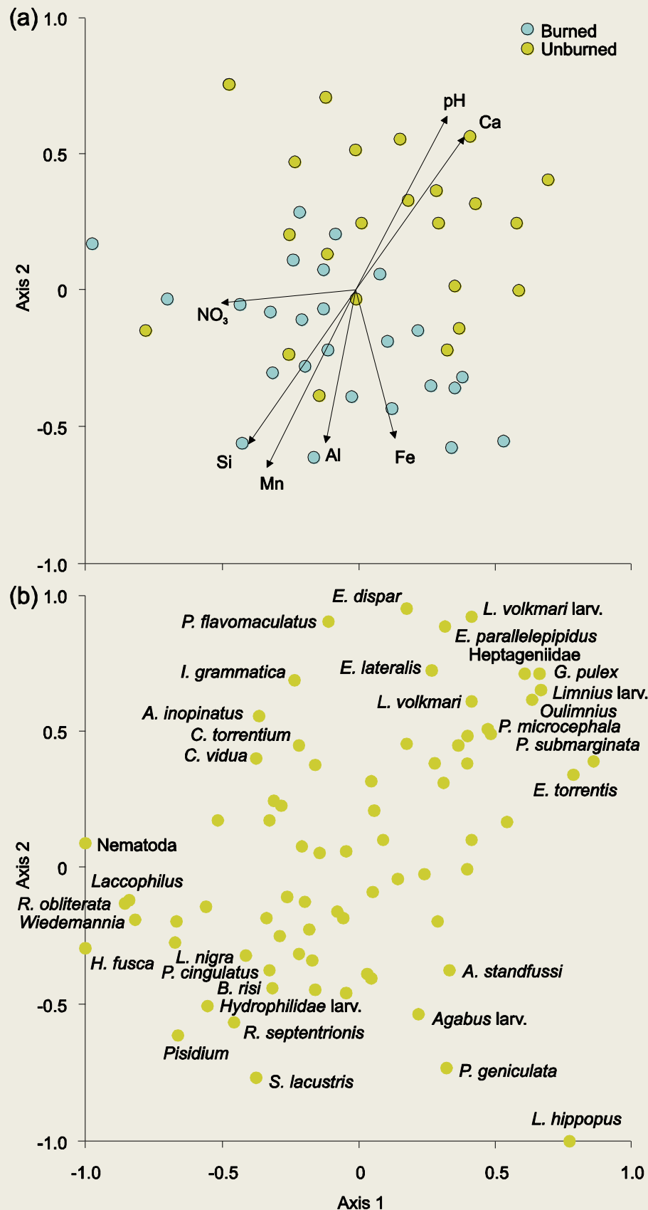
Figure 6.3. (a) NMDS biplot of samples and significantly correlated environmental variable vectors (pH: R^2=0.43 , p=0.001 ; NO 3 (nitrate): R^2=0.20 , p=0.014 ; Al (aluminium): R^2=0.27 , p=0.001 ; Ca (calcium): R^2 = 0.39 , p=0.001 ; Fe (iron): R^2=0.27 , p=0.003 ; Mn (manganese): R^2=0.46 , p=0.001 ; Si (silica): R^2=0.42 , p=0.001 ), and (b) benthic macroinvertebrates.
